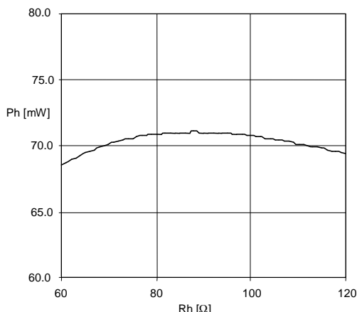
Fig. 3: P_h as a function of R_h . R_{serial} = 88 \Omega and V_{cc} = 5 V
