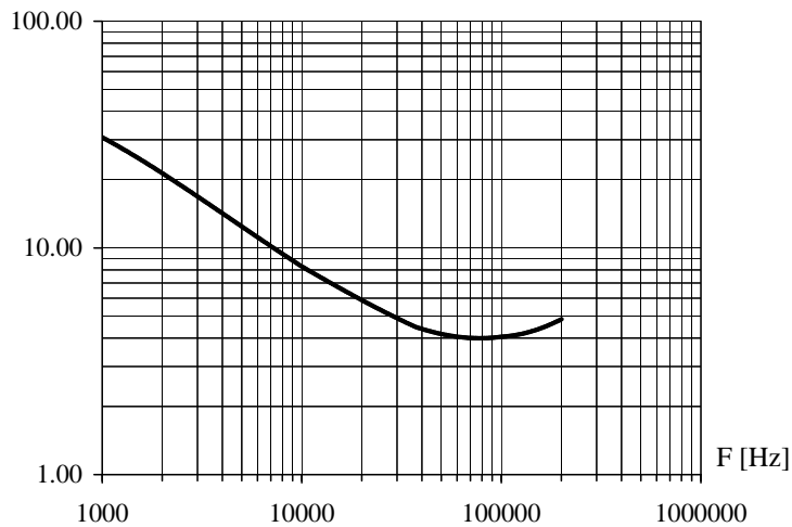
Equivalent serie resistance versus frequency
