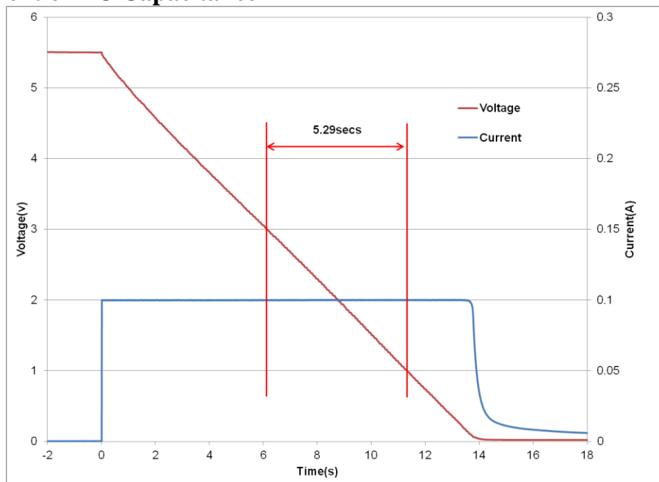
Fig 2: Measurement of DC Capacitance for an HW202
