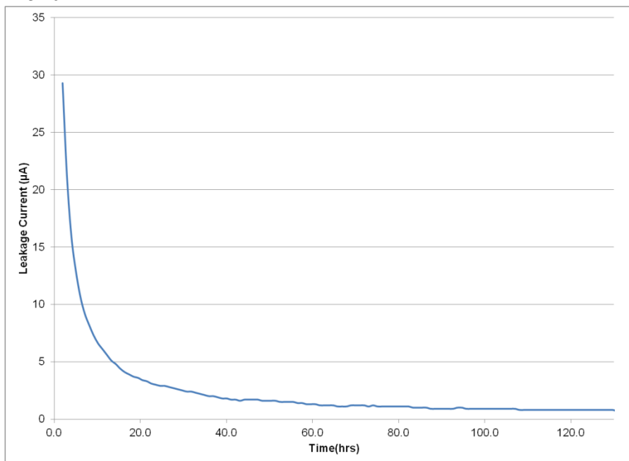
Fig 10: Leakage Current
