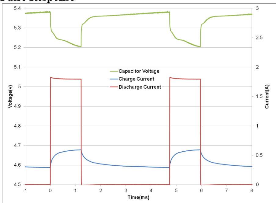
Fig 5: HW202 Pulse Response with GPRS Class 10 Pulse Train
