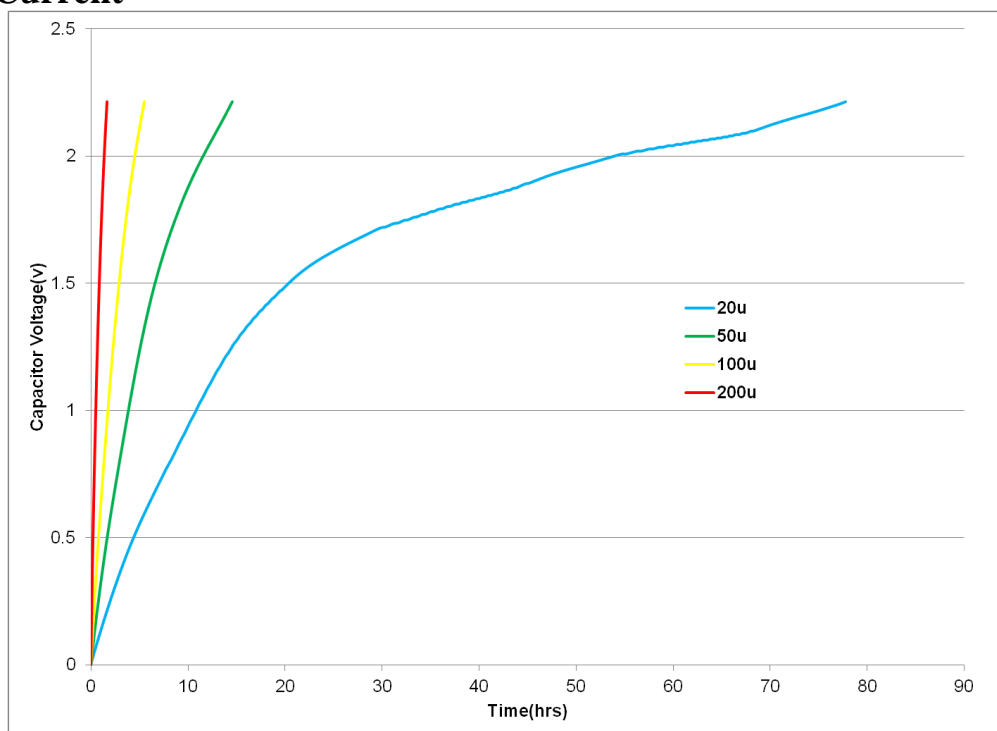
Fig 11: Charging an HW102 with low current
