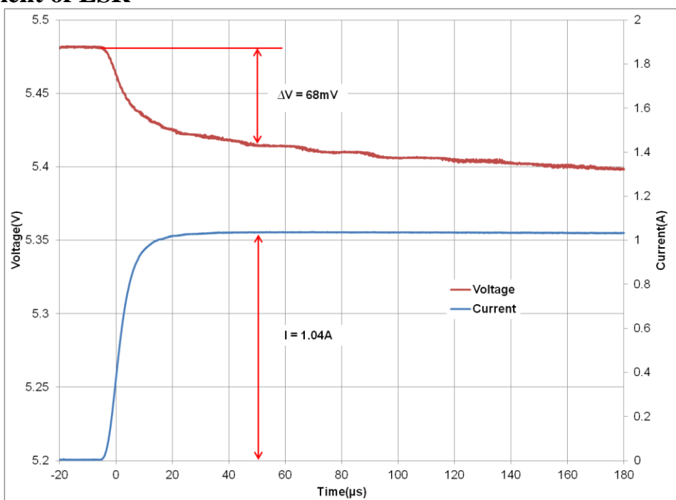
Fig 3: Measurement of ESR for an HW202
