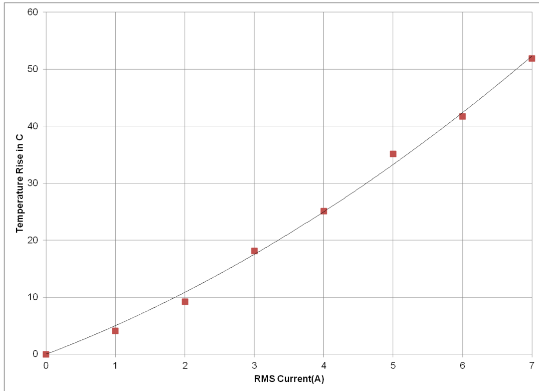
Fig 12: Temperature rise in HW202 with RMS current
