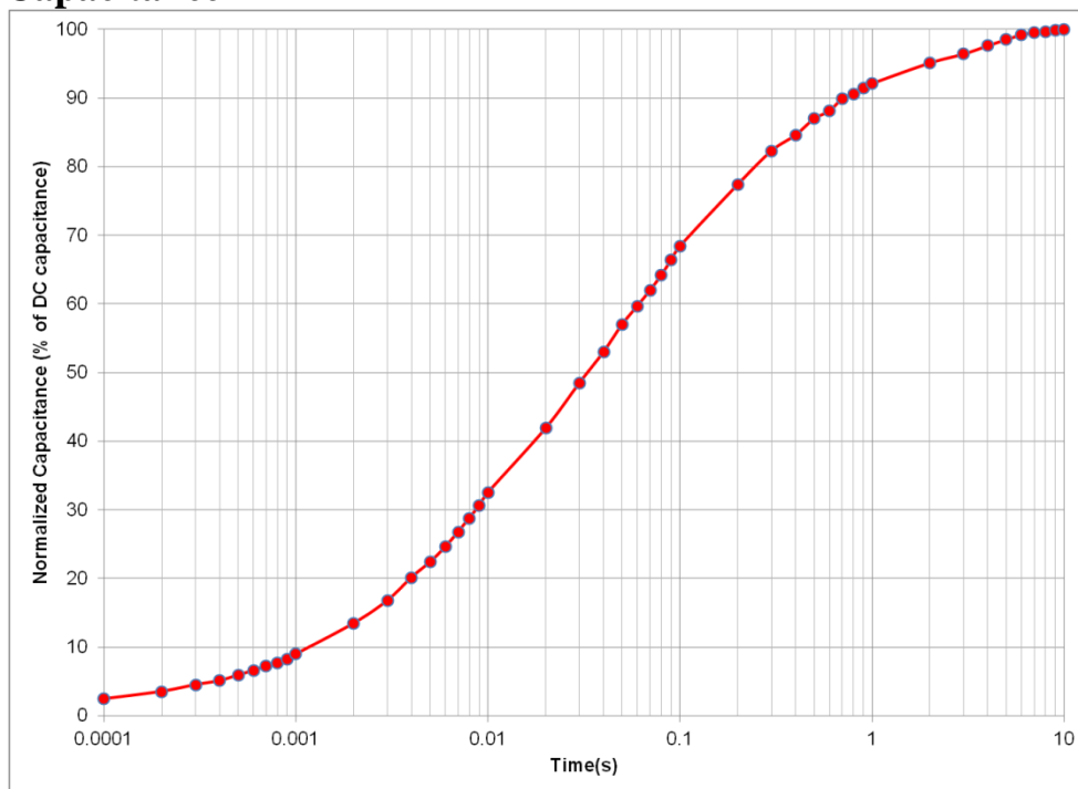
Figure 4: Effective Capacitance
