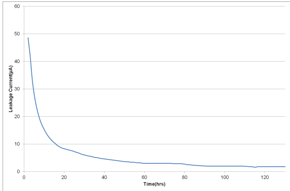
Fig 10: Leakage Current
