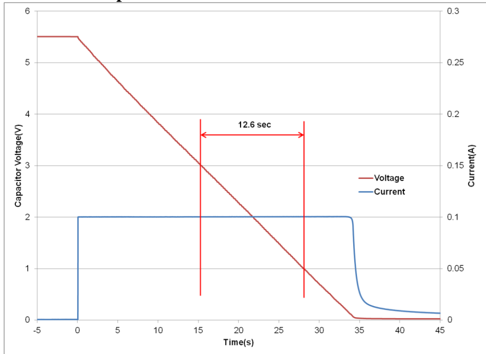
Fig 2: Measurement of DC Capacitance for an HS206
