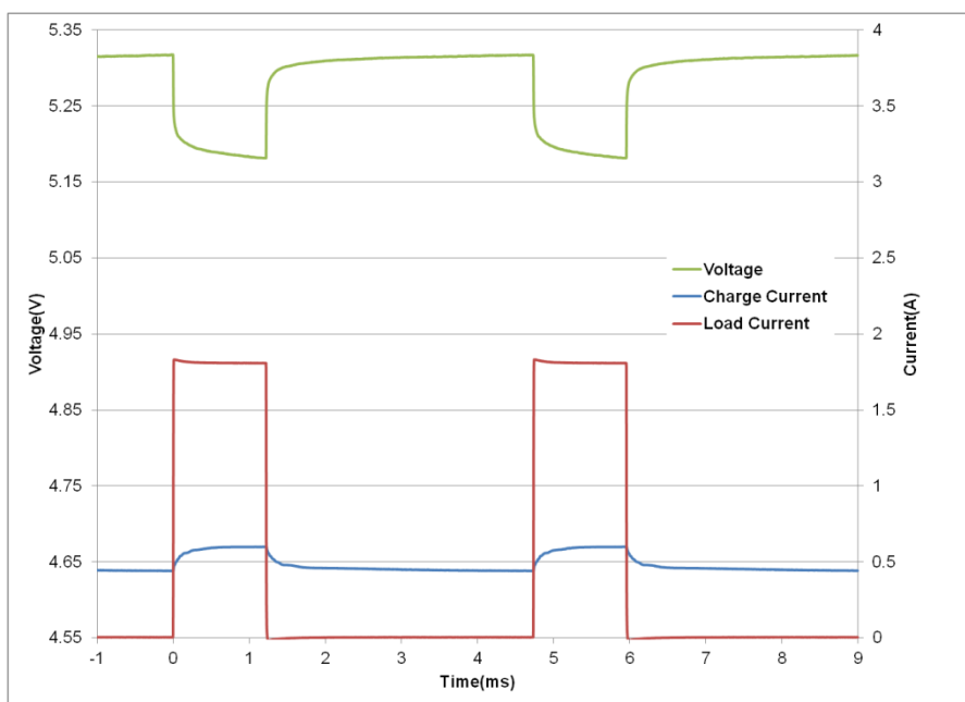
Fig 5: HS206 Pulse Response with GPRS Class 10 Pulse Train
