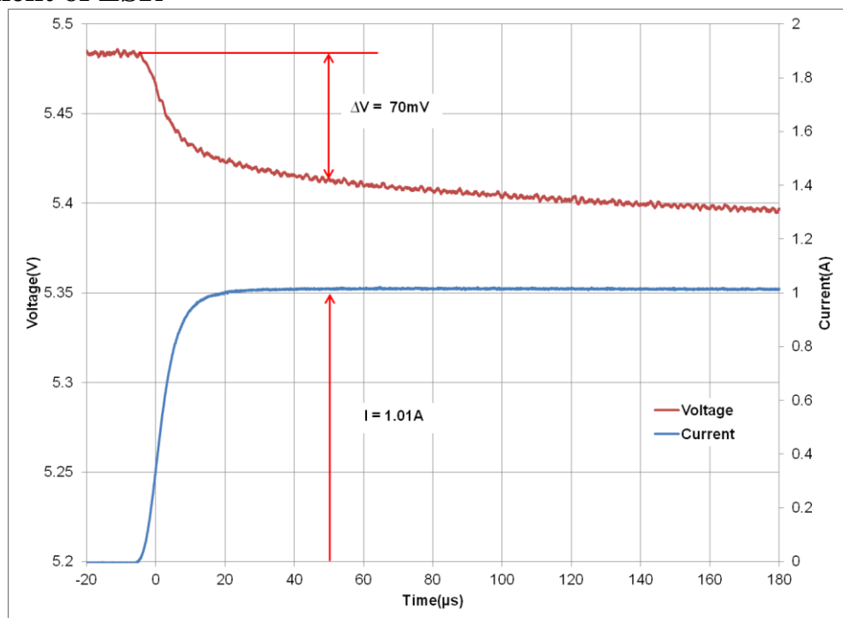
Fig 3: Measurement of ESR for an HS206
