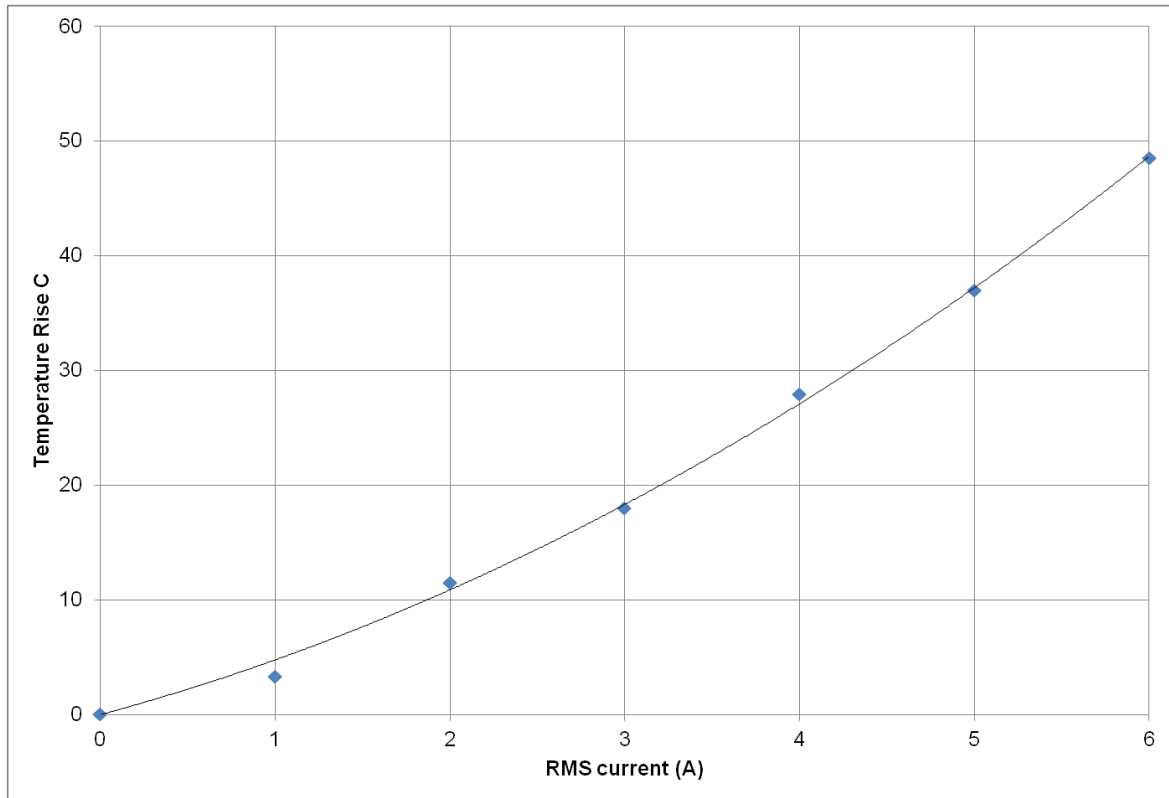
Fig 12: Temperature rise in HS206 with RMS current
