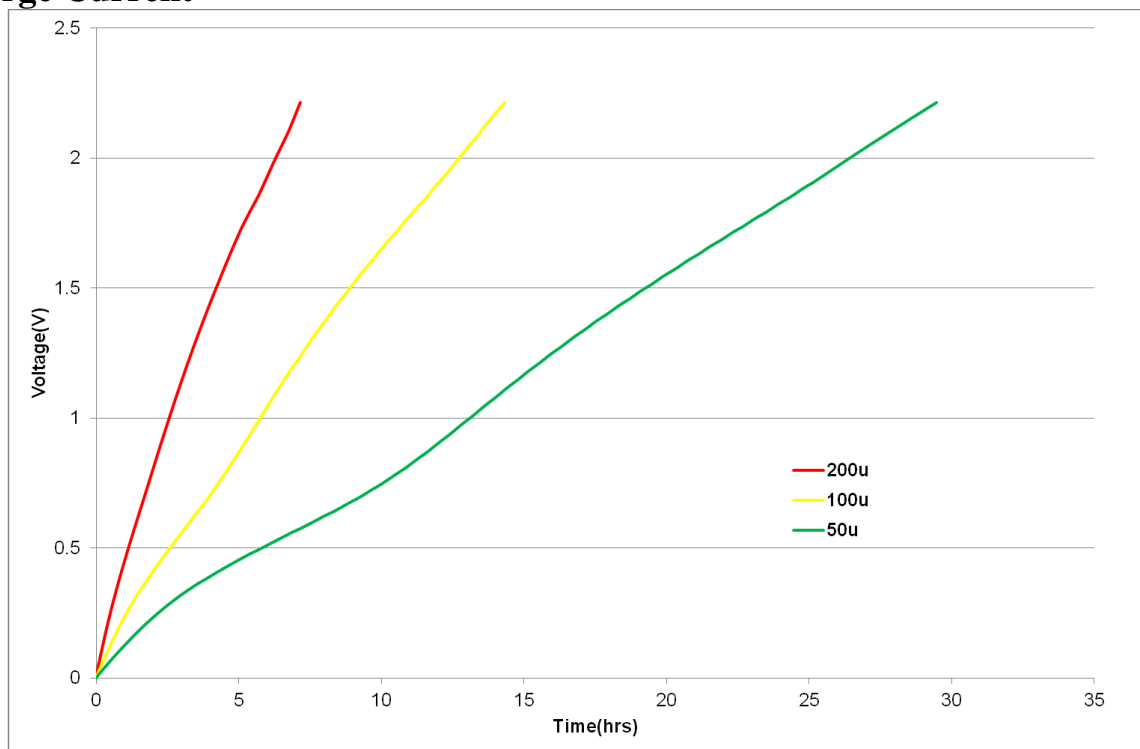
Fig 11: Charging an HS106 with low current
