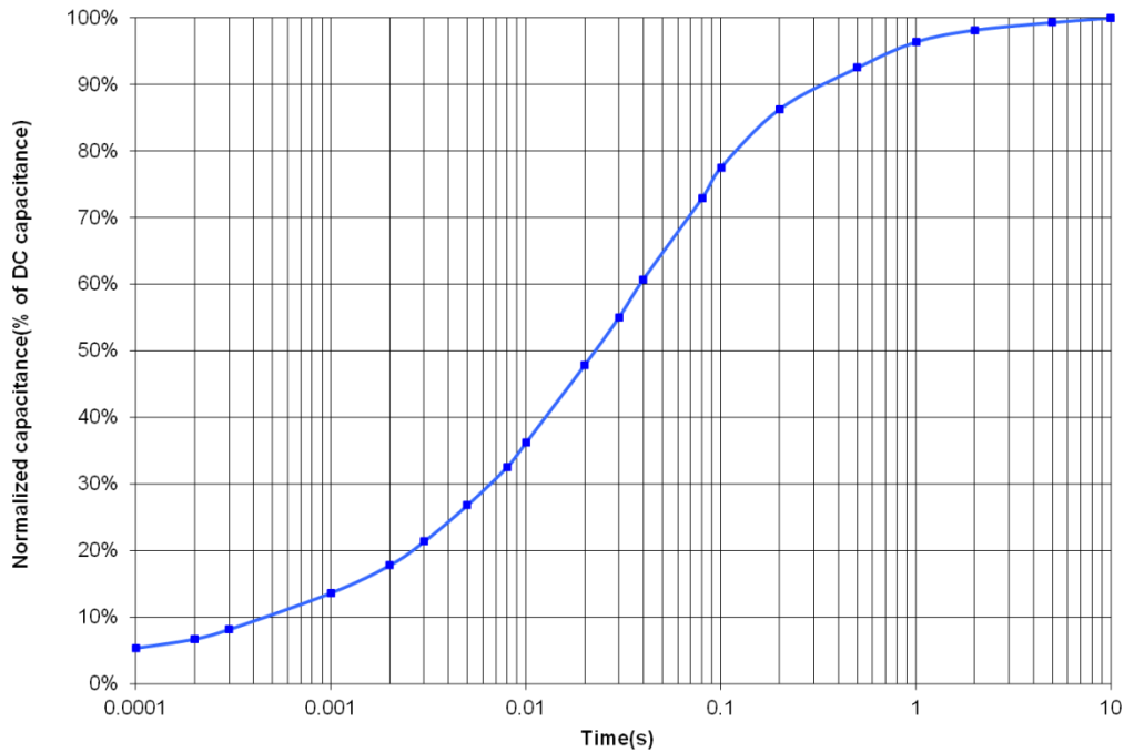
Figure 4: Effective Capacitance
