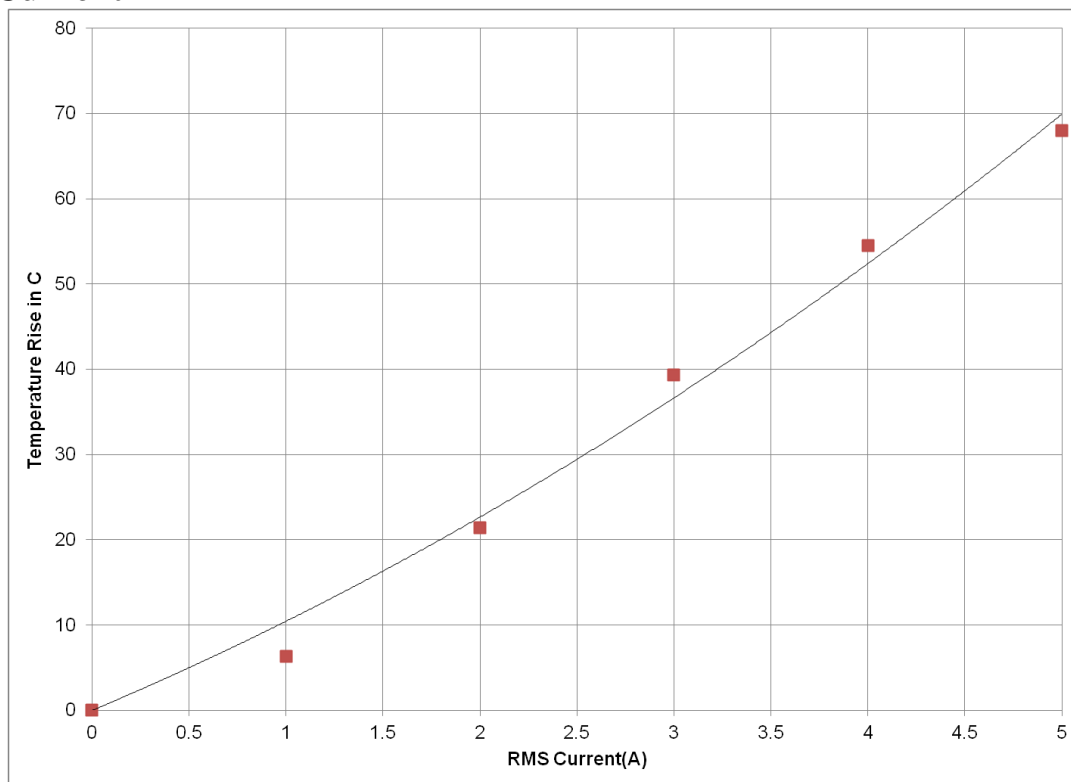
Fig 12: Temperature rise in HA230 with RMS current
