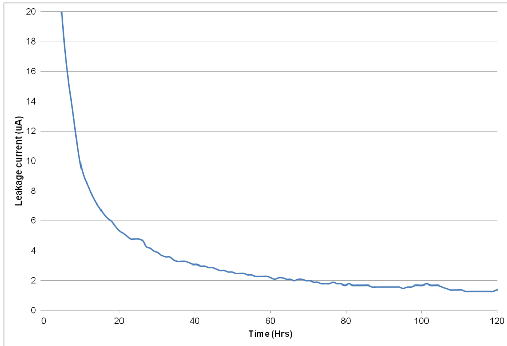
Fig 10: Leakage Current
