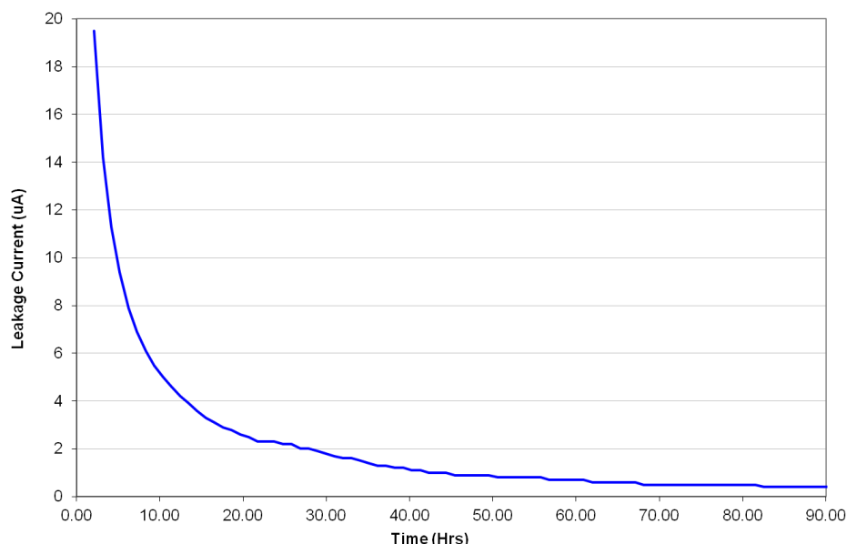
Fig 10: Leakage Current
