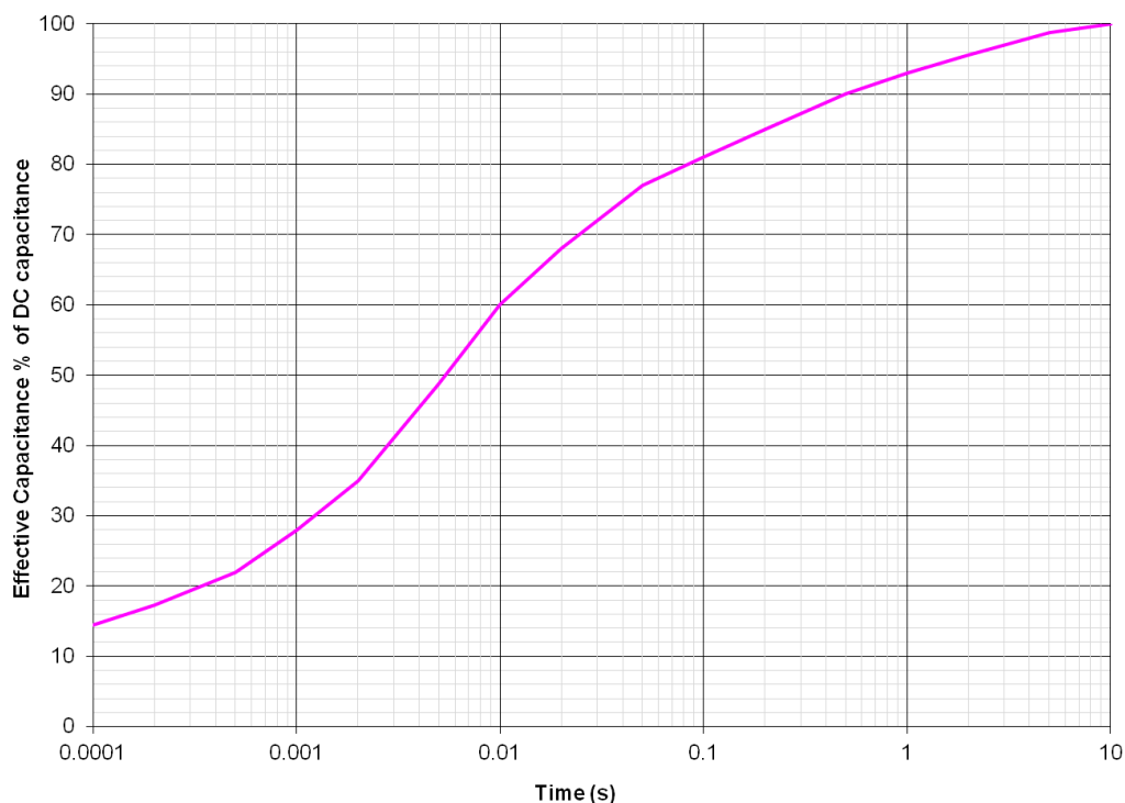
Figure 4: Effective Capacitance
