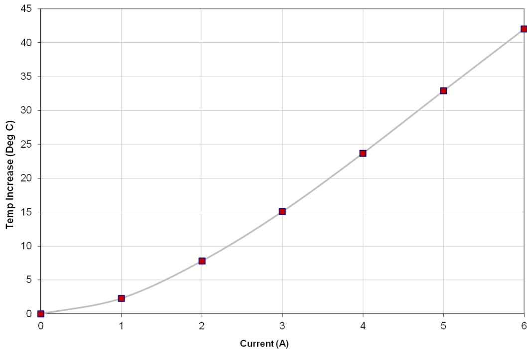
Fig 12: Temperature rise in GW209 with RMS current
