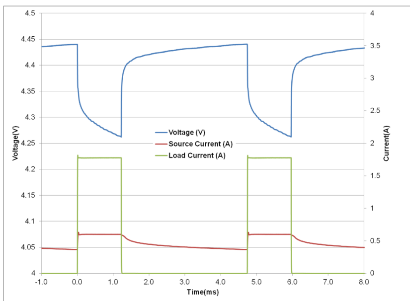
Fig 5: GW209 Pulse Response with GPRS Class 10 Pulse Train
