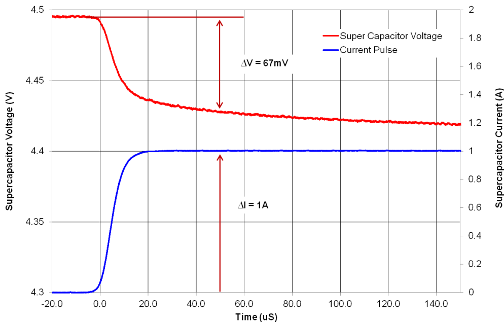
Fig 3: Measurement of ESR for a GW209
