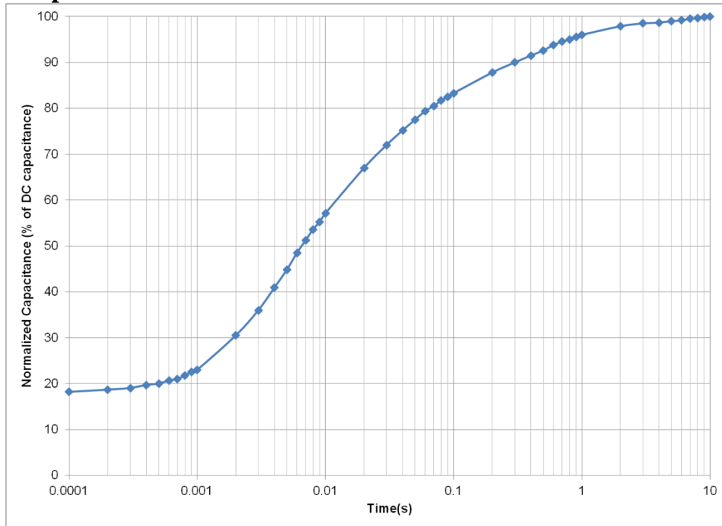
Figure 4: Effective Capacitance
