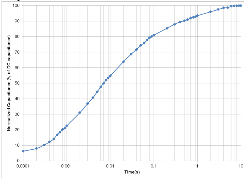
Figure 4: Effective Capacitance
