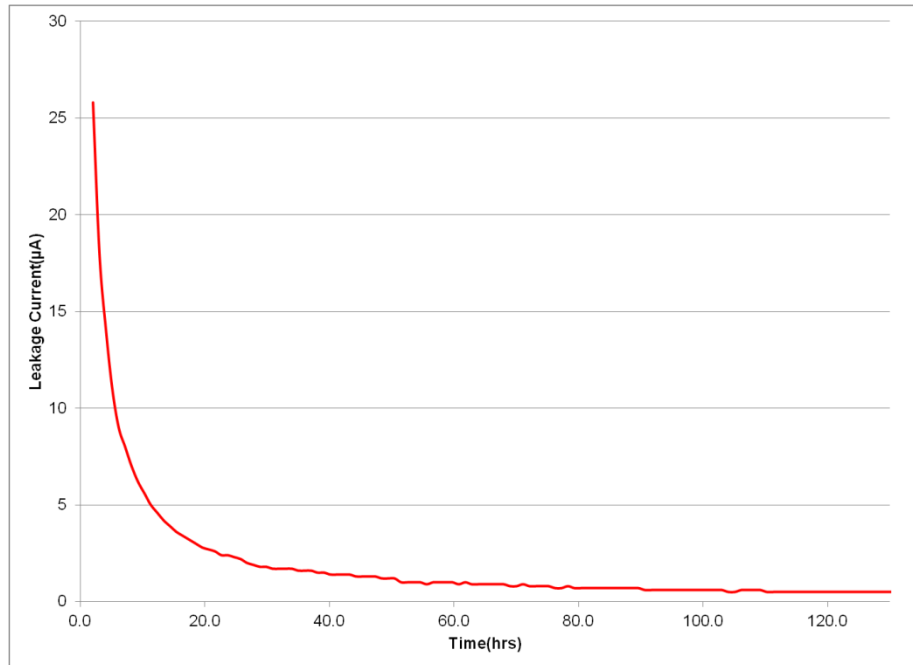
Fig 10: Leakage Current
