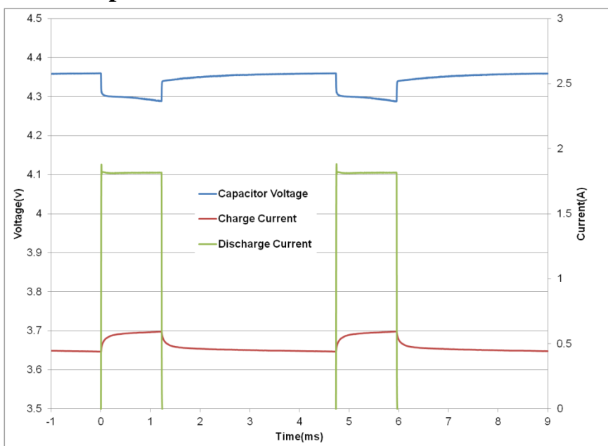
Fig 5: GW202 Pulse Response with GPRS Class 10 Pulse Train
