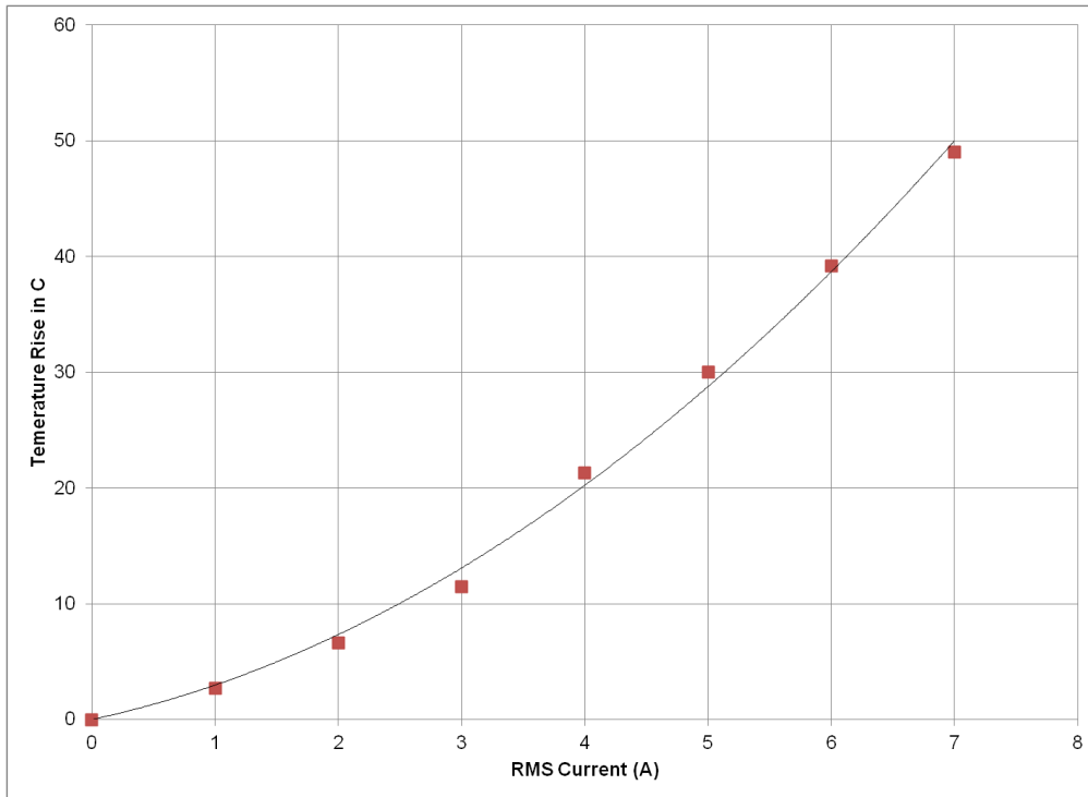
Fig 12: Temperature rise in GW202 with RMS current
