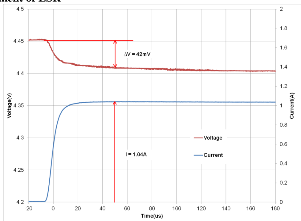
Fig 3: Measurement of ESR for a GW202
