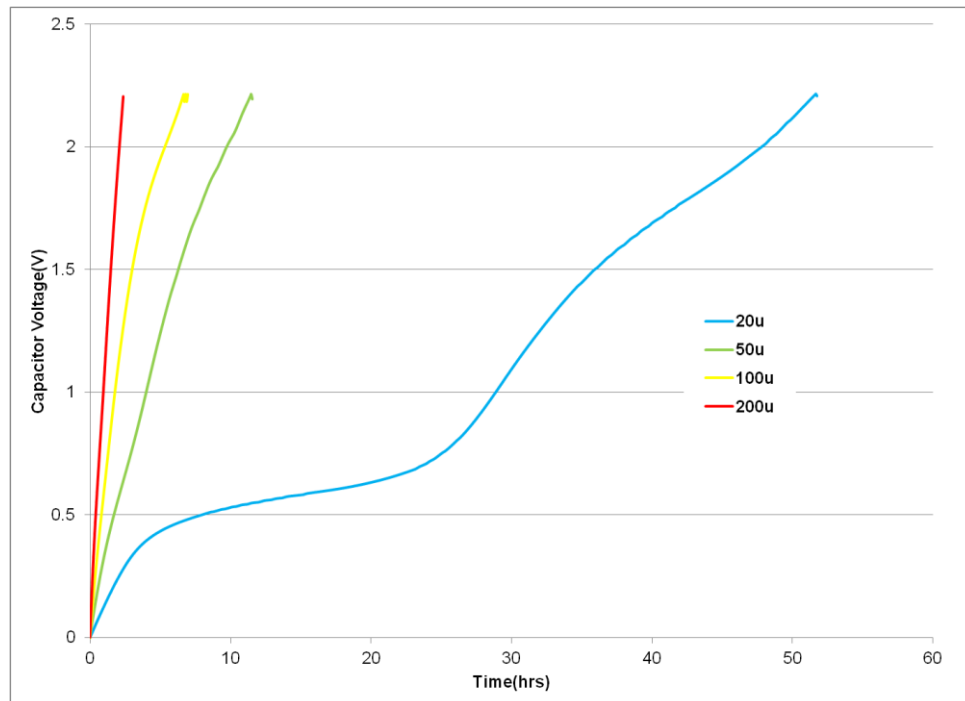
Fig 11: Charging an GW102 with low current
