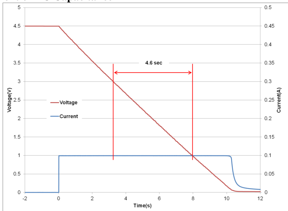
Fig 2: Measurement of DC Capacitance for a GW202
