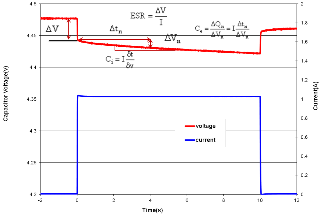
Figure 1: Effective capacitance, instantaneous capacitance and ESR for a GS208
