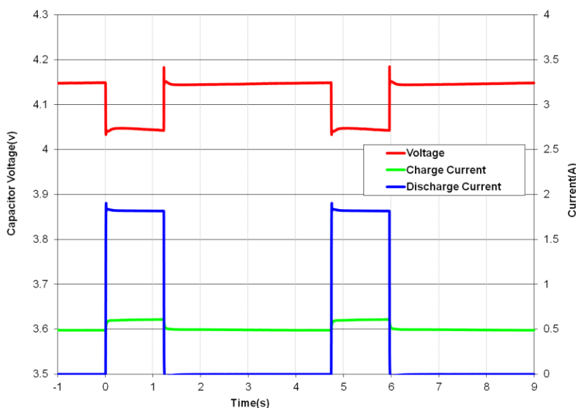
Fig 5: GS208 Pulse Response with GPRS Class 10 Pulse Train
