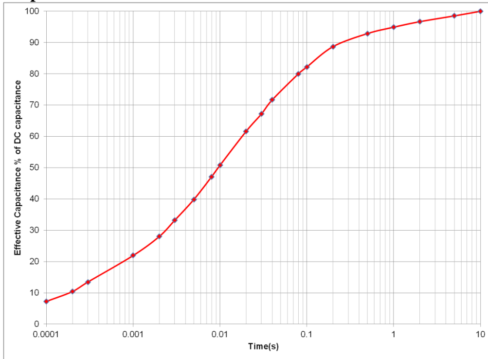
Figure 4: Effective Capacitance
