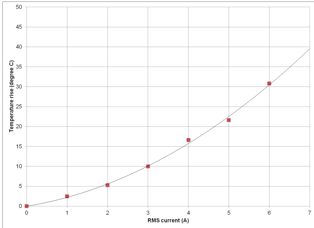
Fig 12: Temperature rise in GS208 with RMS current
