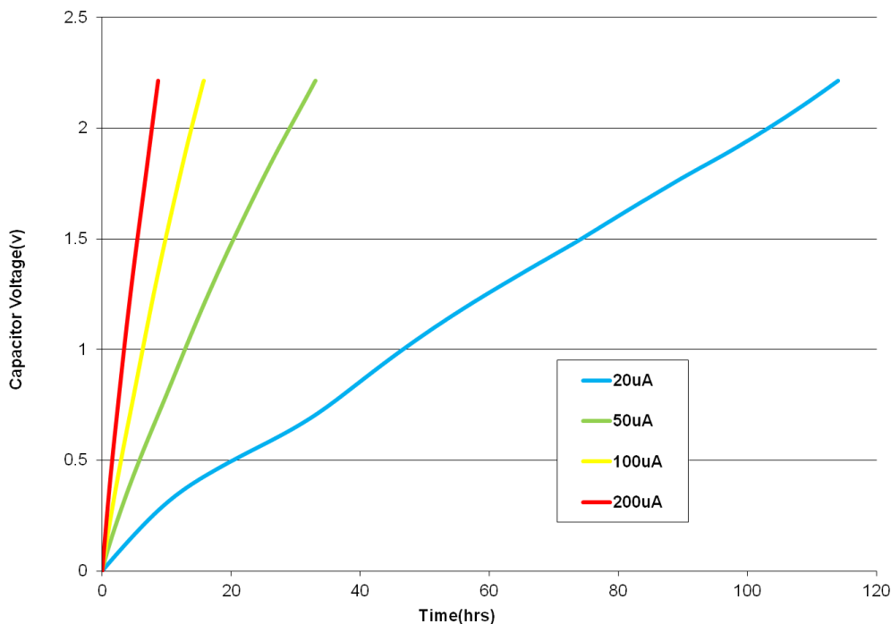
Fig 11: Charging an GS108 with low current
