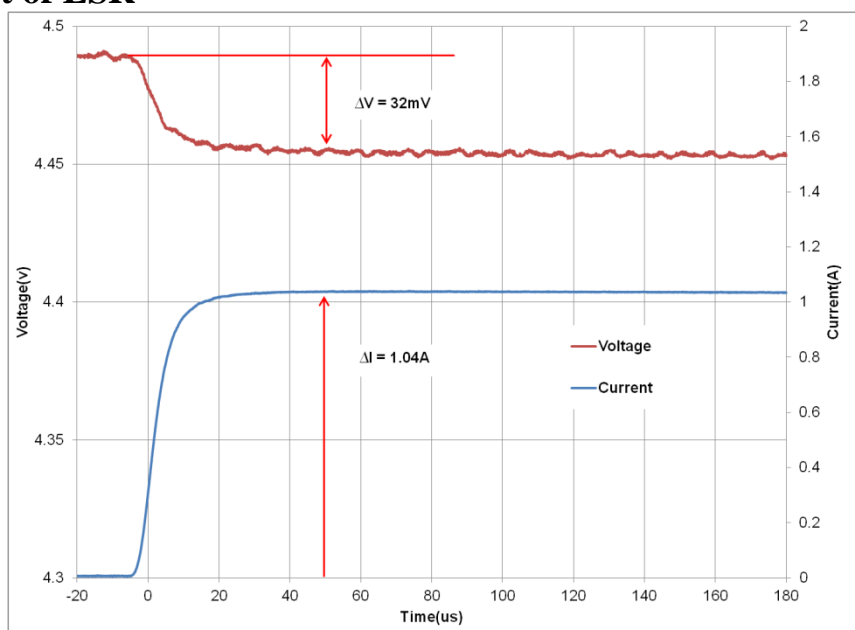
Fig 3: Measurement of ESR for a GS208
