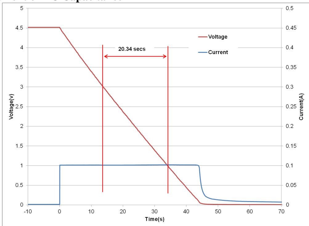
Fig 2: Measurement of DC Capacitance for a GS208
