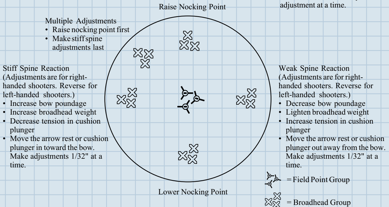
Fig. 20 Broadhead Tuning
