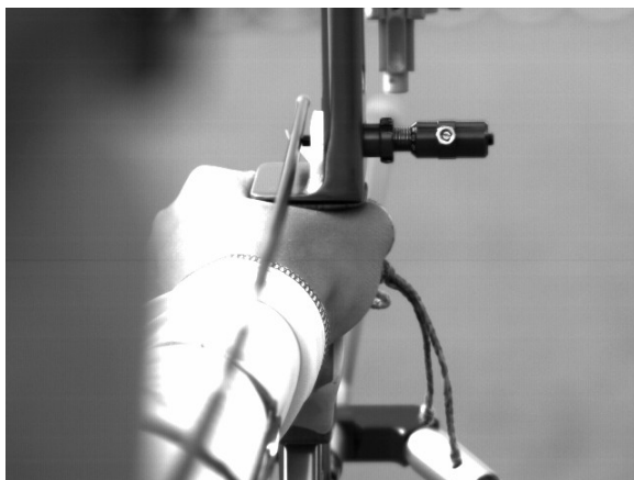
Arrow pushes against Plunger, moving plunger in about .5 mm
