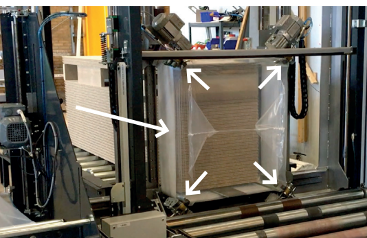
The stretch hood packaging process
