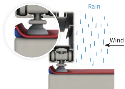
Fabric with anti-drip system
