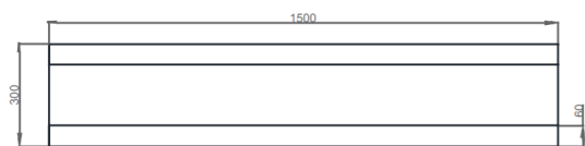
Truckværn
