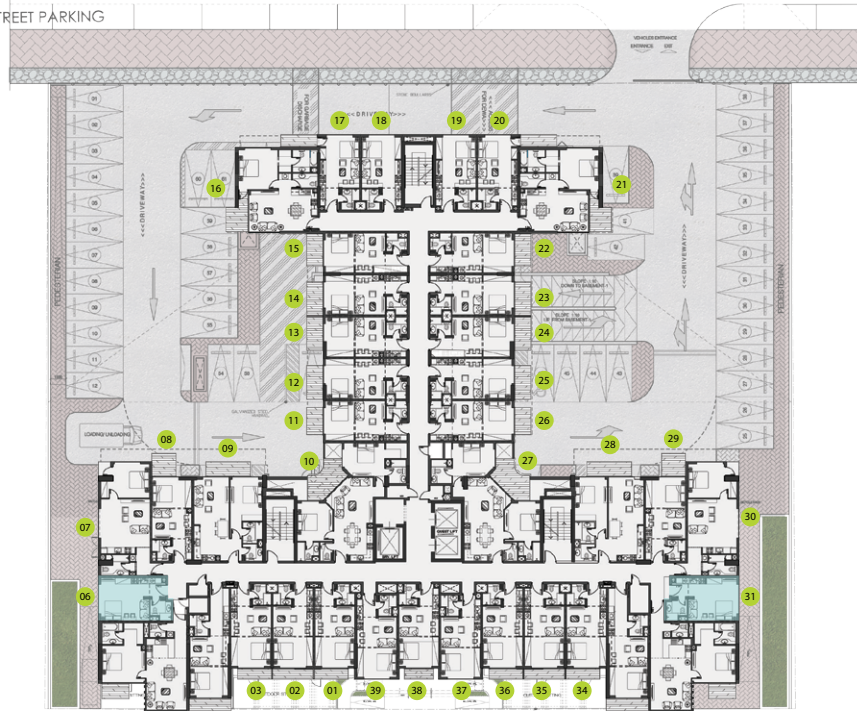
GROUND FLOOR NUMBER OF PARKING:44 SHEIKH MOHAMMED BIN ZAYED ROAD
