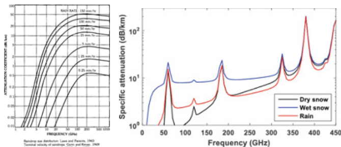
(14) Attenuation versus frequency for rain intensity and snow
