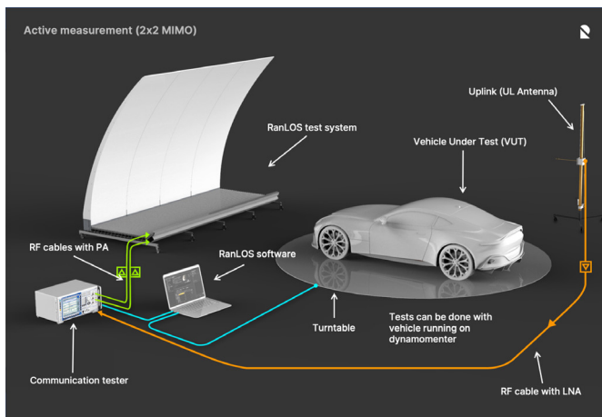
(20) RanLOS BeamForce 42 setup in active configuration to measure throughput and receiver threshold in a 2x2 MIMO communication system. Note that the threshold is affected by the level of the disturbances
