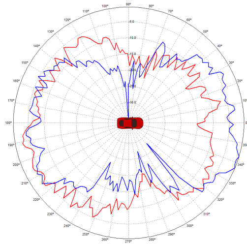
(15) Antenna radiation pattern comparison
