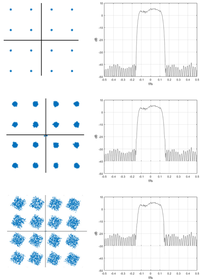
(7) Signal-to-noise ratio (SNR) from good to worse in a 16 QAM constellation diagram
