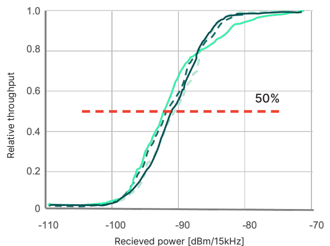
(8) Threshold, the received power level when 50% of the communication signal is received without errors.
