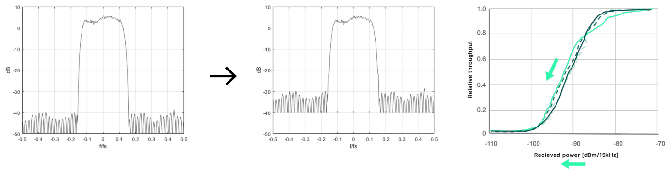
(9) Signal-to-noise ratio (SNR) from good to worse (left) results in a lower relative throughput that can be shown in the throughput diagram (right)
