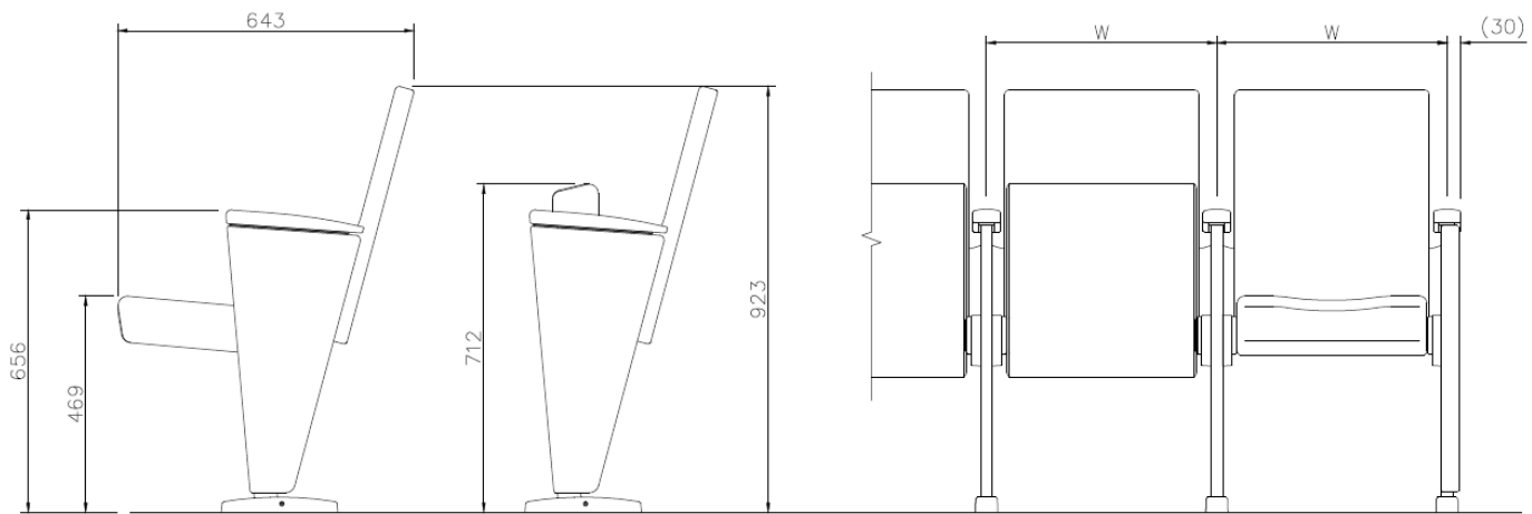
All dimensions are in mm and are nominal. Seat height is taken at seat centre.
