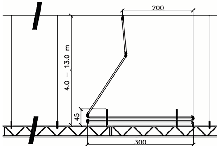
Hinge element
