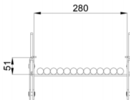
CROSSECTION
