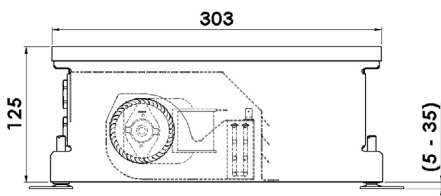
CROSS SECTION
