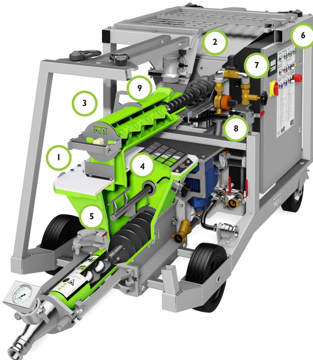
Applying shotcrete
