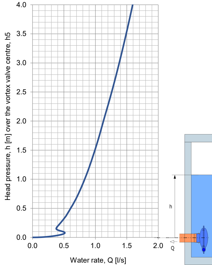
Hydraulic curve
