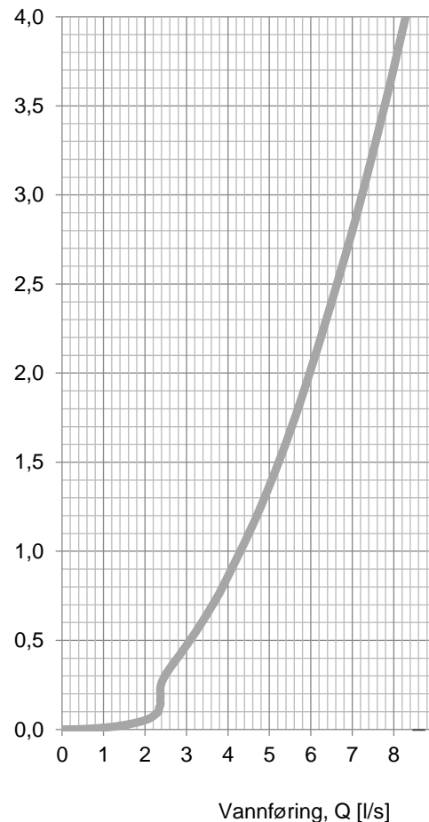
Hydraulisk kurve
