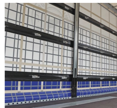
POWER CURTAIN body without support laths and lath brackets for shorter loading and unloading times. Built-in anti-theft protection through steel wires incorporated into the tarpaulin to prevent intentional cutting.
