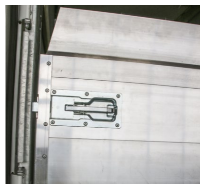
Locking the bridge into the corner stanchions allows the entire body width to be used.
