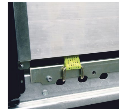
Lashing eyes along the entirety of the frame , with clearance under the lath storage (in conjunction with the pallet stop).
