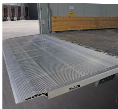
Spring-supported bridge reduces physical demands when operating.
