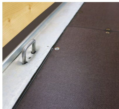
Stable plywood floor with a 5,460 kg stacker axle load.
