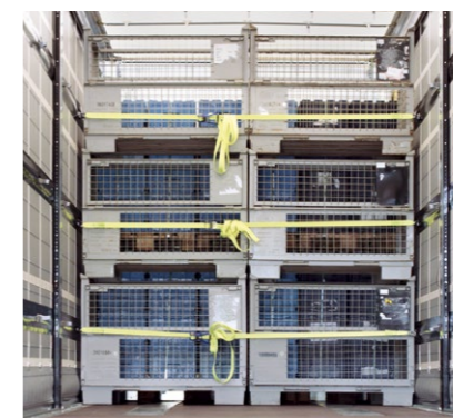
Rear load securing with stitched-on tarpaulin loops for tensioning belts or safety tarpaulins. Arranged in three rows above each other, the loops have a securing force of up to 7,500 daN with partial loads (2,500 daN per row).
