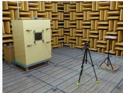
Anechoic Chamber
