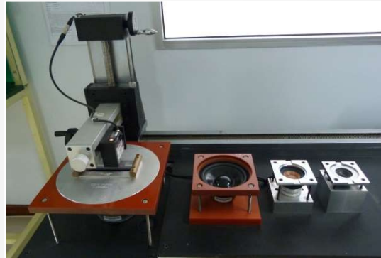
FO Cone Paper Tester
