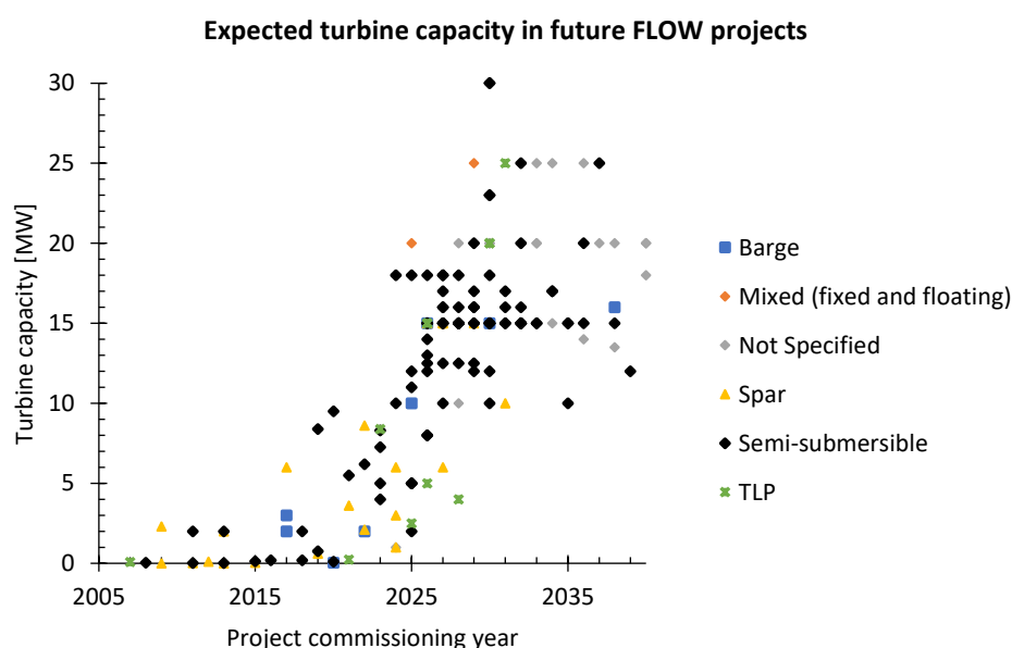
Figure 4.1 – Turbine capacity of FLOW projects in the pipeline [10], shown by type of floating foundation (hull) they are expected to employ. Data from a database licenced to Gavin & Doherty Geosolutions by TGS 4C Offshore in November 2023. Any low values are for test-scale projects.
