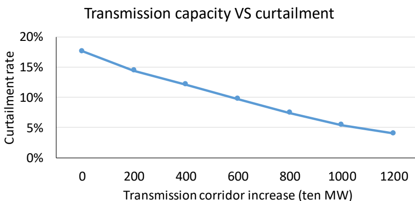
Figure 76. Influence of increased transmission grid flexibility to wind power curtailments in an example power system in China (Source: SGERI).
