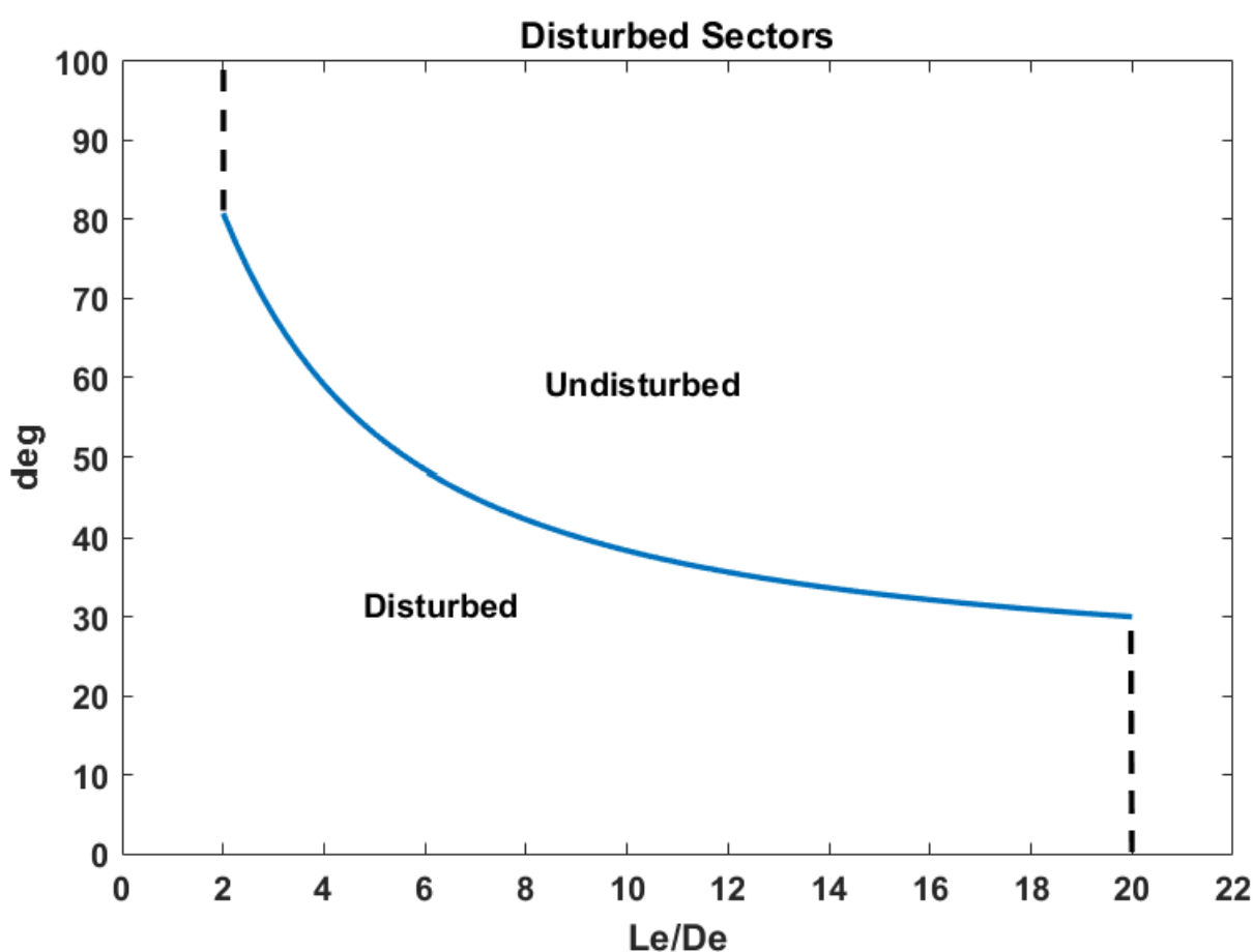
Figure 10. Disturbed flow as a function of L_e/D_e and degrees Graphic courtesy of Raymond Byrne based on IEC 61400-12-1 Annex A.
