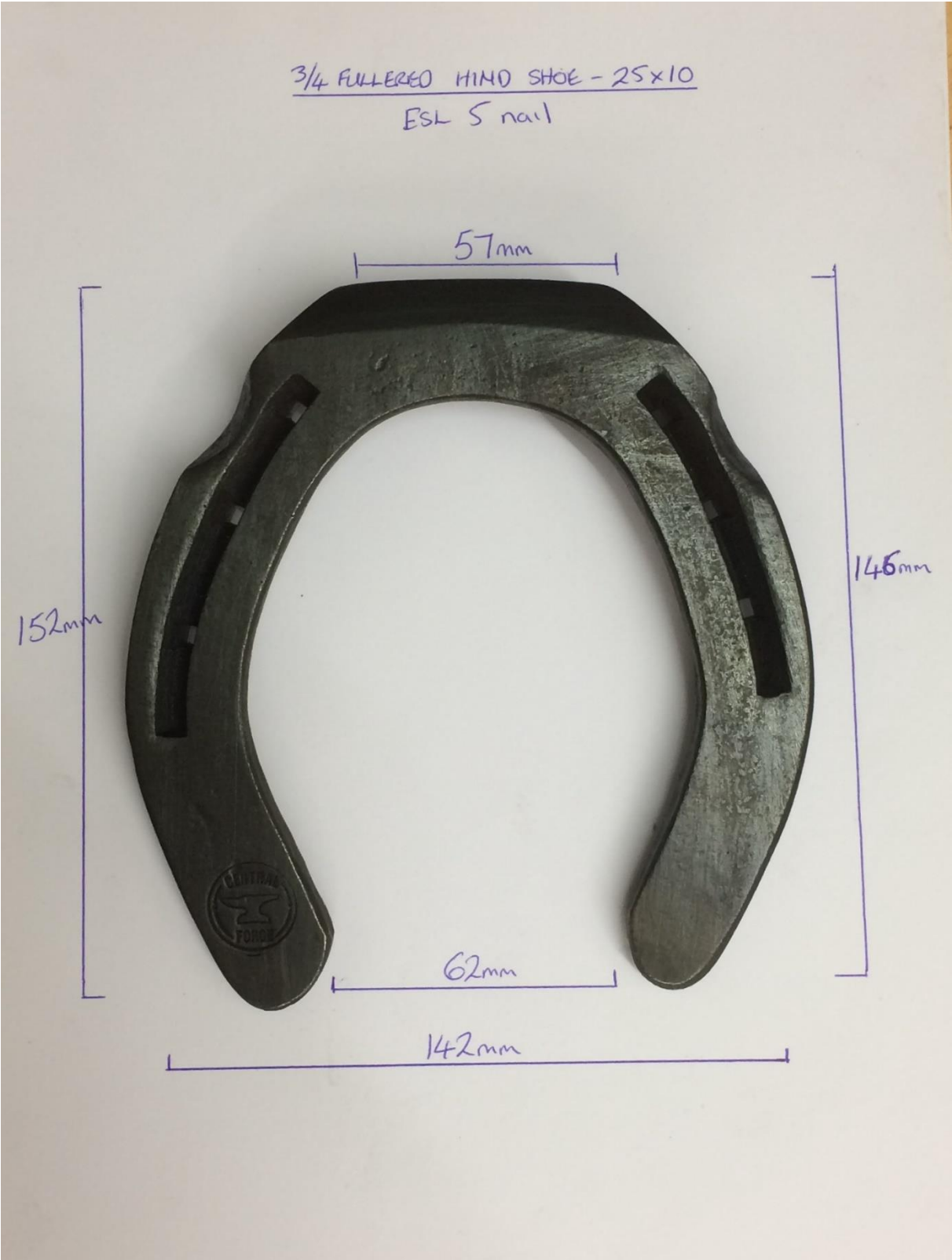
Sko B: 3/4 fullered hind shoe
