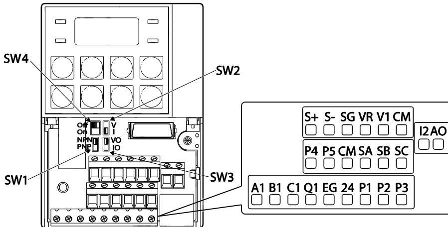
<Standard E/A>
