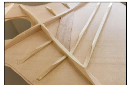
X-type bracing pattern (spruce)
