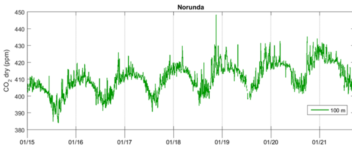
Figure 4. CO 2 measurements 2015-2021 (source: ICOS).
