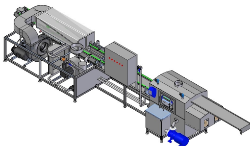
WASHING MACHINE WITH BLOWING AND DRYING SECTION
