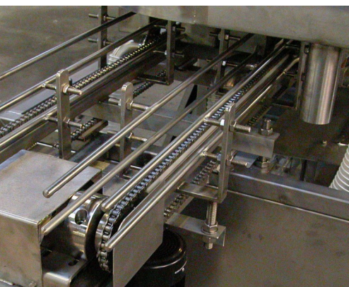
WASHING SECTION WITH TWO-LINE INFEED
