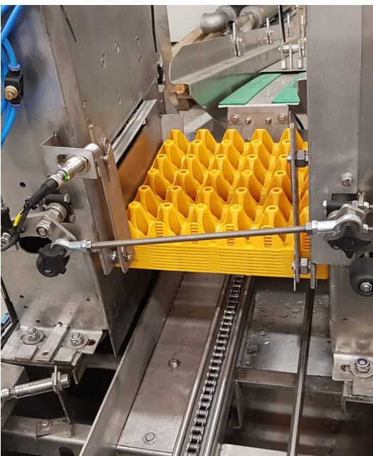
DE-STACKER FOR EGG TRAYS
