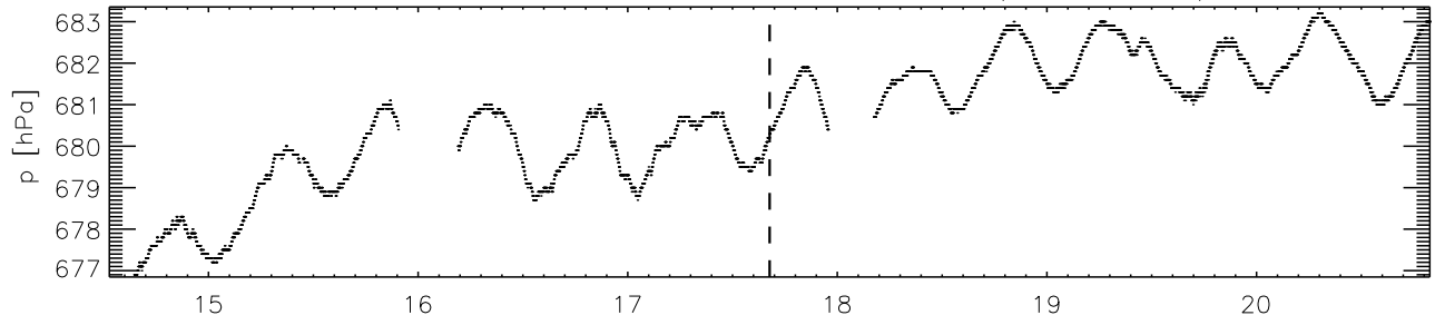
Met conditions at MLO near Jan 18 2012 (JD 2455945)
