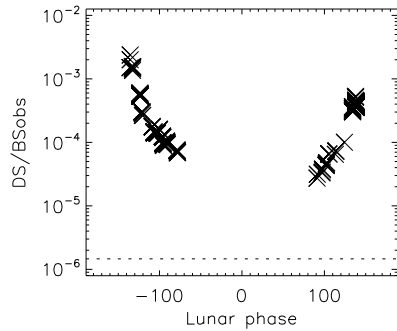
EFMCLEANED _VE2_ Non-UNIFORM no skypatch VE2_ Non-UNIFORM no skypatch
