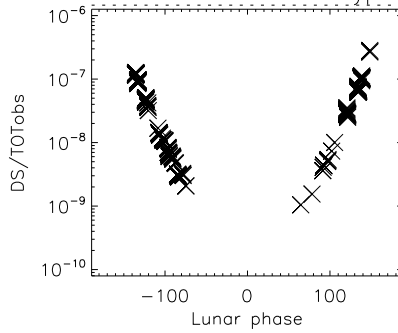
EFMCLEANED _V_ Non-UNIFORM no skypatch _V_ Non-UNIFORM no skypatch
