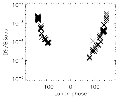
EFMCLEANED _JRCUT_ Non-UNIFORM no skypatch JRCUT_ Non-UNIFORM no skypatch
