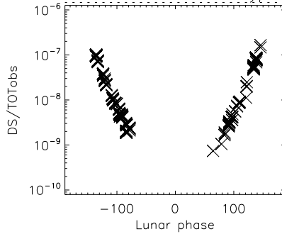
EFMCLEANED _VE1_ Non-UNIFORM no skypatch VE1_ Non-UNIFORM no skypatch
