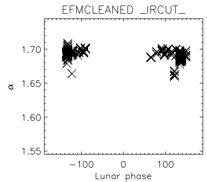
EFMCLEANED _JRCUT_ Non-UNIFORM no skypatch JRCUT_ Non-UNIFORM no skypatch
