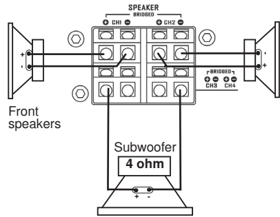
Rear or front stereo speakers connected to channels 1 / 2 and subwoofer to channels 3 / 4.
