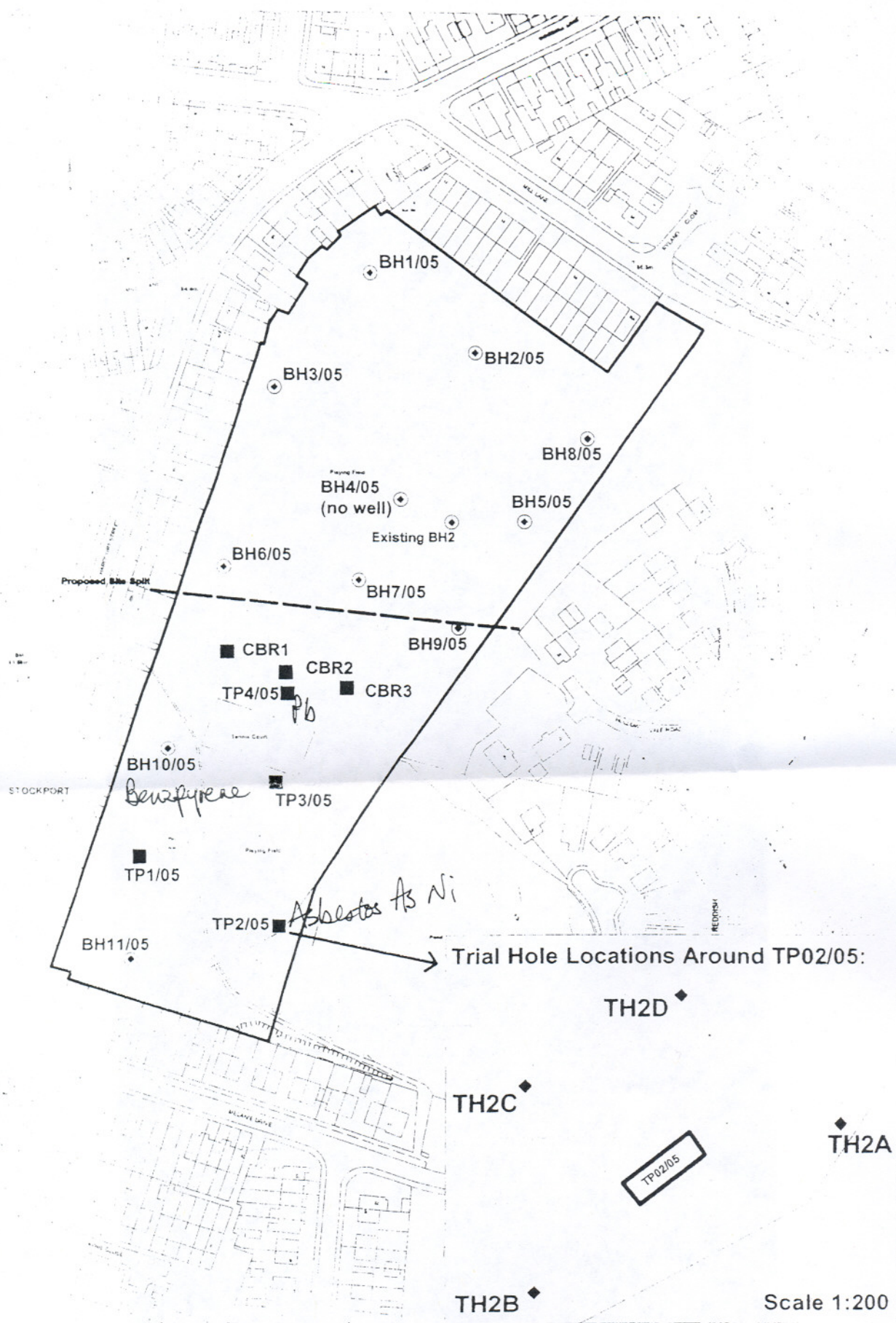
Figure 2. Harcourt Street Playing Field Site Investigation Layout
