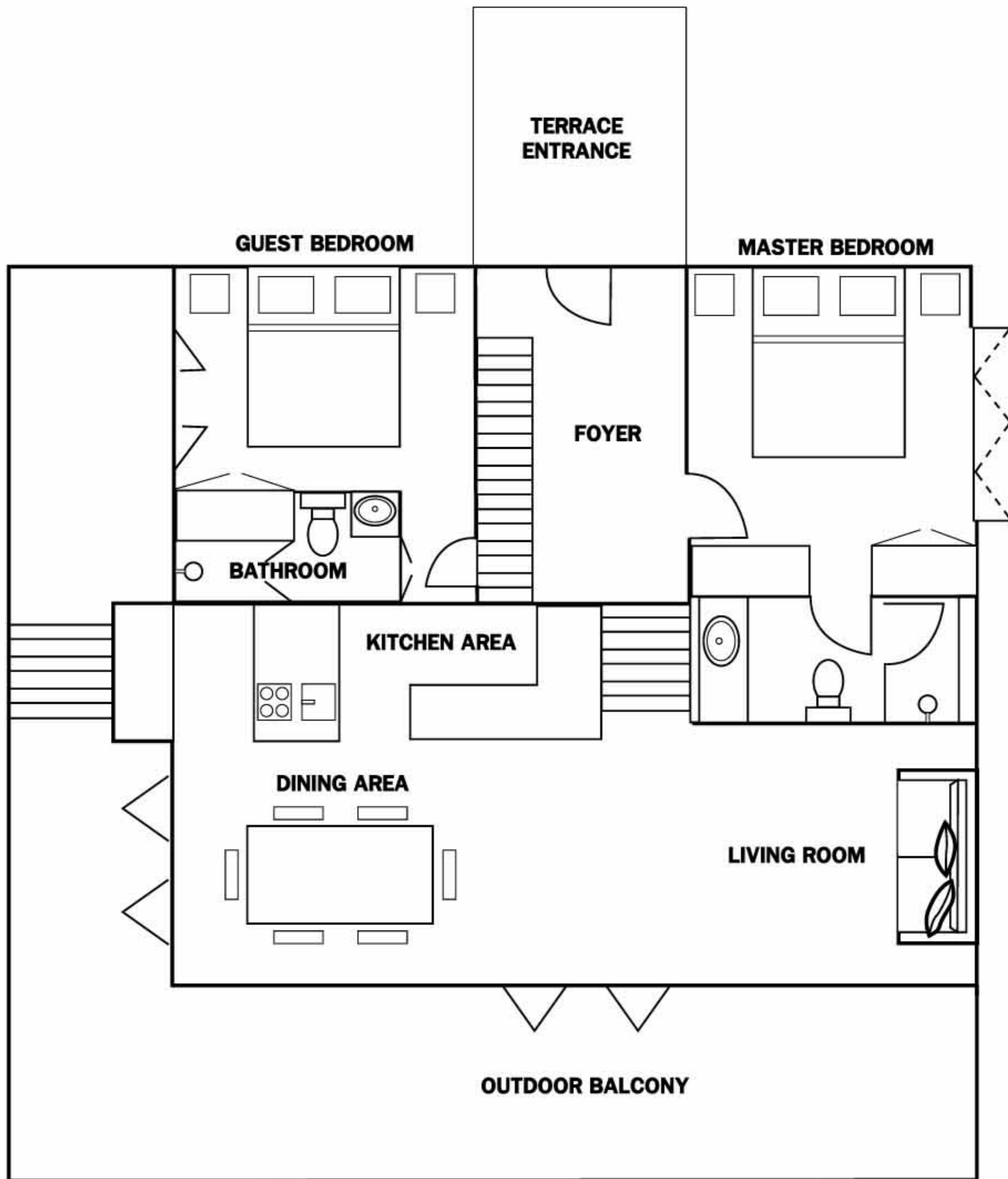
1 st FLOOR BAAN RAJAPRUK
